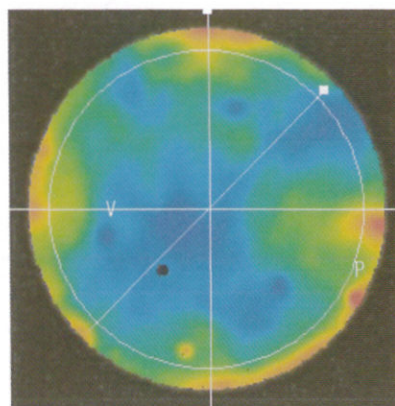
X断面 (PV=0.165 \mu m RMS=0.046 \mu m)
